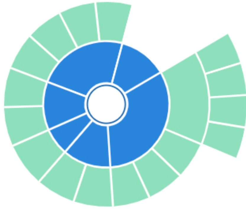
Discussion Topology
